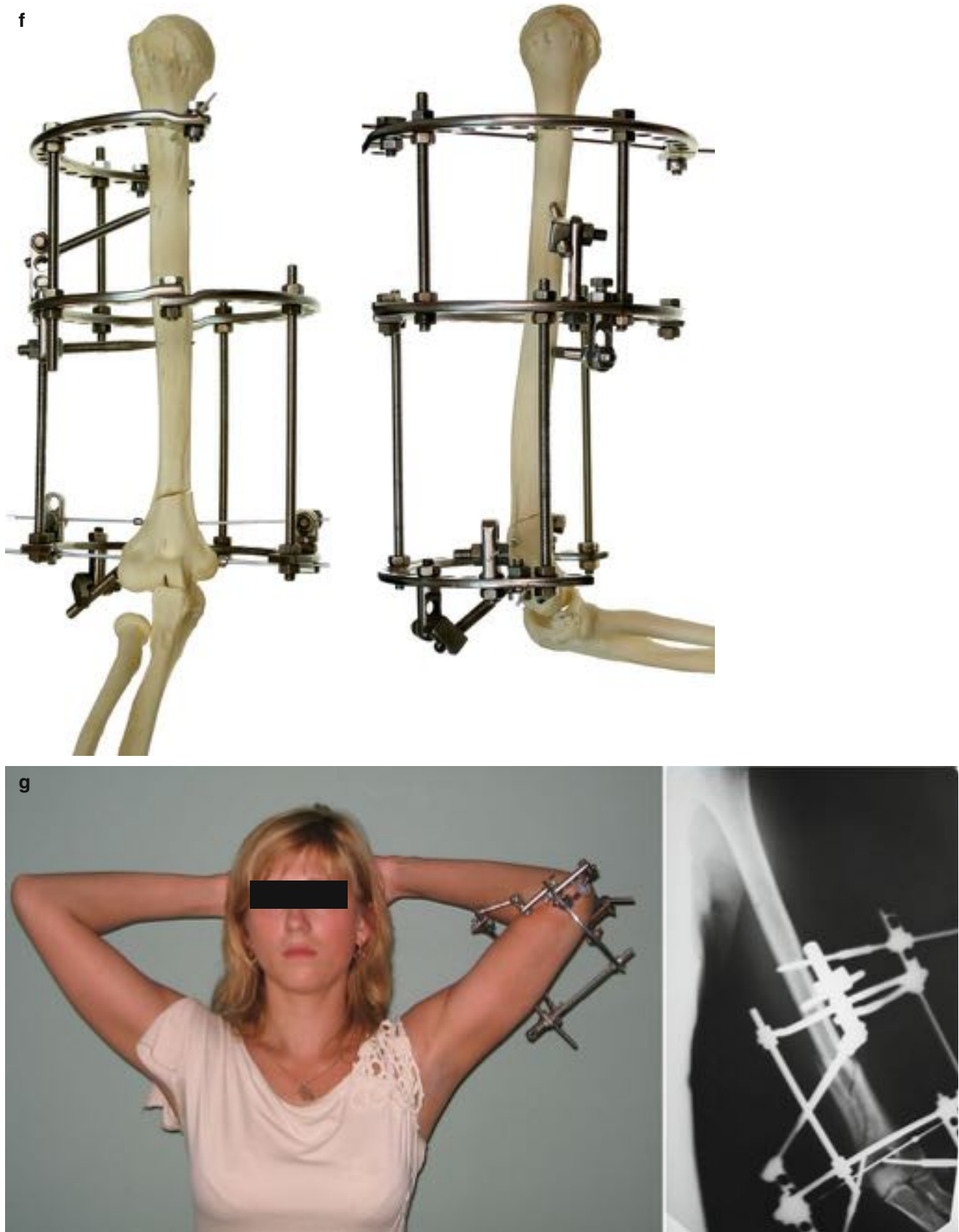
Fig. 10.16 (continued) (f) Insertion and fixation to supports of stabilizing half-pins III,9,120 and VIII,8,120. Elimination of the diastasis. Dismantling of skeletal traction. (g) Patient after module transformation
